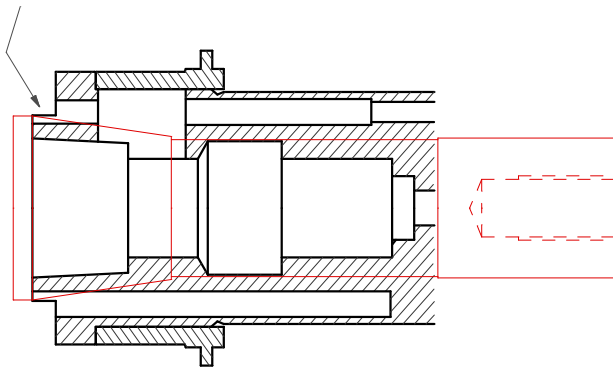
SPINDLE WITH R8 COLLET
